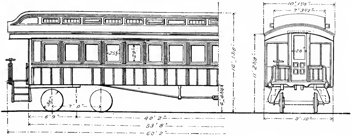
Fig. 155. PASSENGER COACH. PENNSYLVANIA RAILROAD. Seating capacity, 64 persons. Weight, 65,600 lbs. (Details are shown in Figs. 435-443.)
